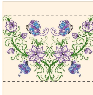
Floral_elegance_10-8x8.dst 7.87x5.53 inches; 22,061 stitches 8 thread changes; 8 colors
