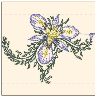
Timeless_iris_09-4x4.dst 3.90x2.90 inches; 7,082 stitches 5 thread changes; 5 colors
